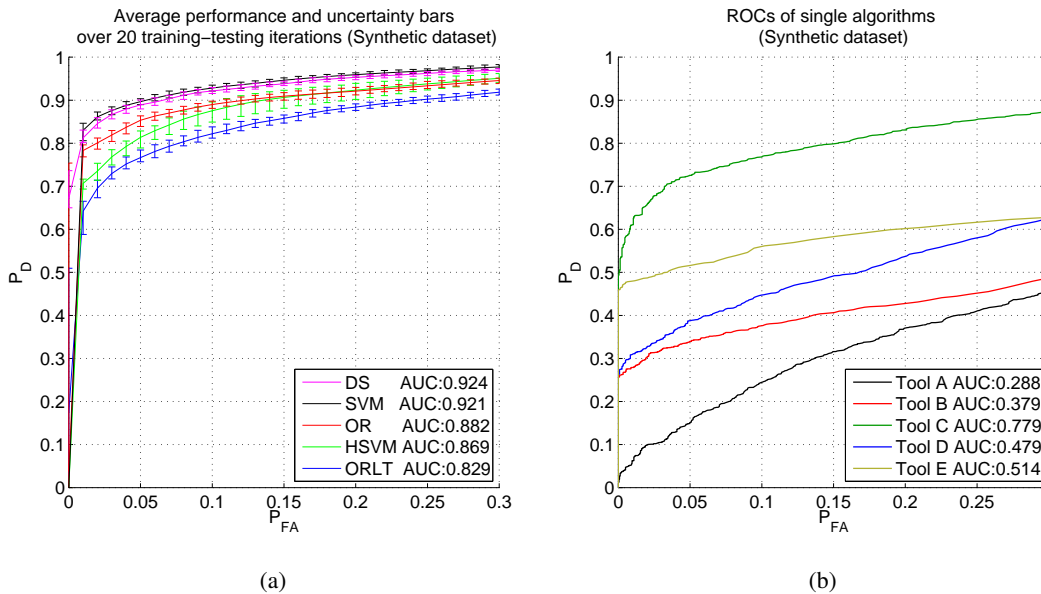
Fig. 6. Results on the synthetic test dataset both using the decision fusion methods (a) and each algorithm separately (b). For all methods involving a training phase, we plot the average performance along with uncertainty bars, showing the maximum and minimum values obtained. AUC values are normalized to the considered interval.
