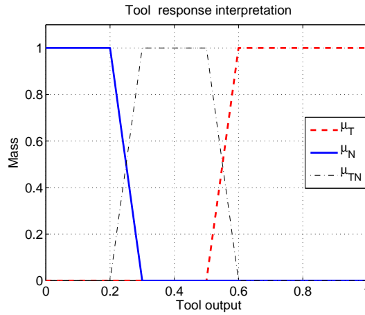
Fig. 1. An example of mapping the tool answer to mass assignments. Such an example is typical for tools featuring a good separation between positive and negative examples: most training examples yield very low ( < 0.2 ) or high ( > 0.6 ) values, while nothing is observed in the middle range. Therefore, should the tool provide 0.5 as output, we can not say anything about the class of the sample (i.e., we have only doubt)
