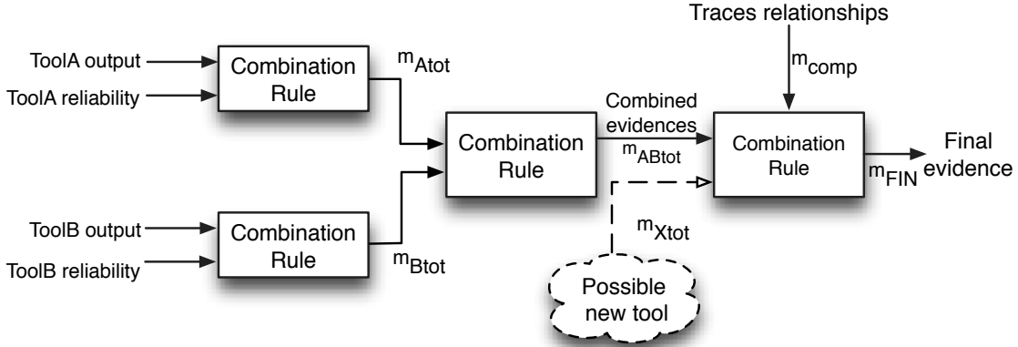
Fig. 2. Block diagram of the proposed fusion approach. Notice that, when a new tool becomes available (represented in the dashed cloud), its BBA directly enters the final stage of the fusion, without needing to recombine information from previous tools.
