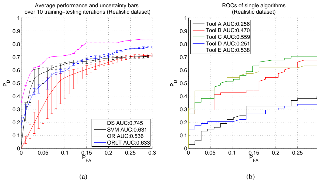
Fig. 7. Results on the realistic test dataset both using the decision fusion methods (a) and each algorithm separately (b). Curves and AUC values have the same meaning of those in Figure 6.
