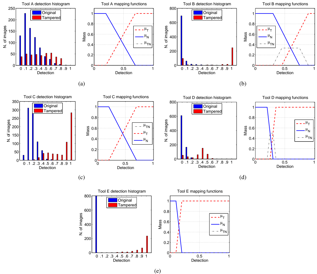
Fig. 5. For each tool, the histogram of detection values on training dataset are shown on the left image. Right images show how this histogram is interpreted to define a mapping from tool detection value ( x -axis) to mass assignment ( y -axis). See eq. 6 for an explanation of each line meaning.
